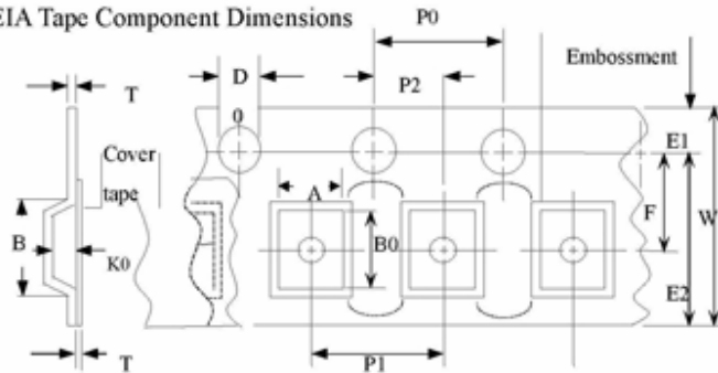
EIA Tape Component Dimensions
